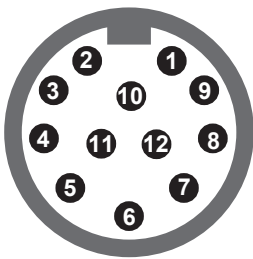
Advanced Connection Type (M12, 12 pins, Male)
