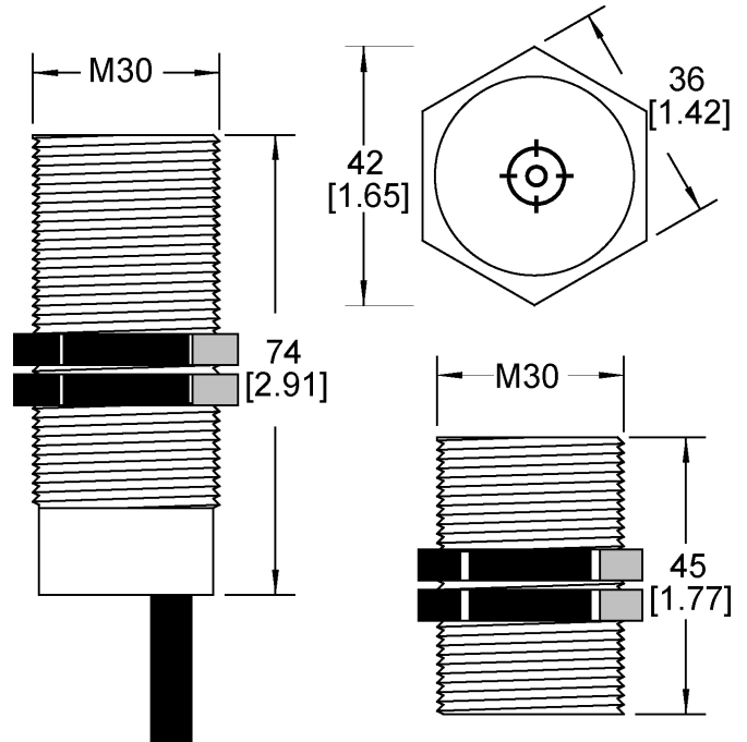
SWITCH
