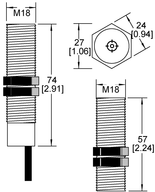
SWITCH
