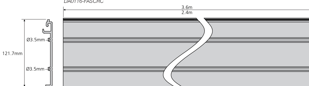
DA0116-FASCRC
